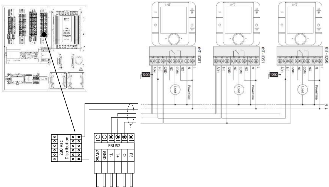
Figure 5.14. Example of connection of thT terminals.
